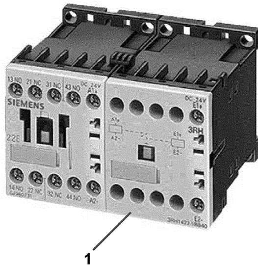
RELAY WITH MECH. LATCHING
