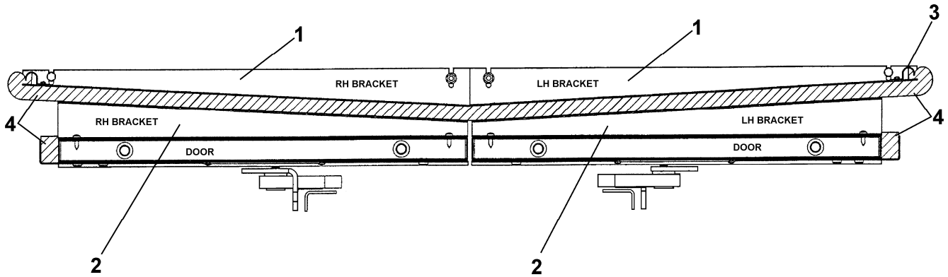
(Car Doors Top View)
