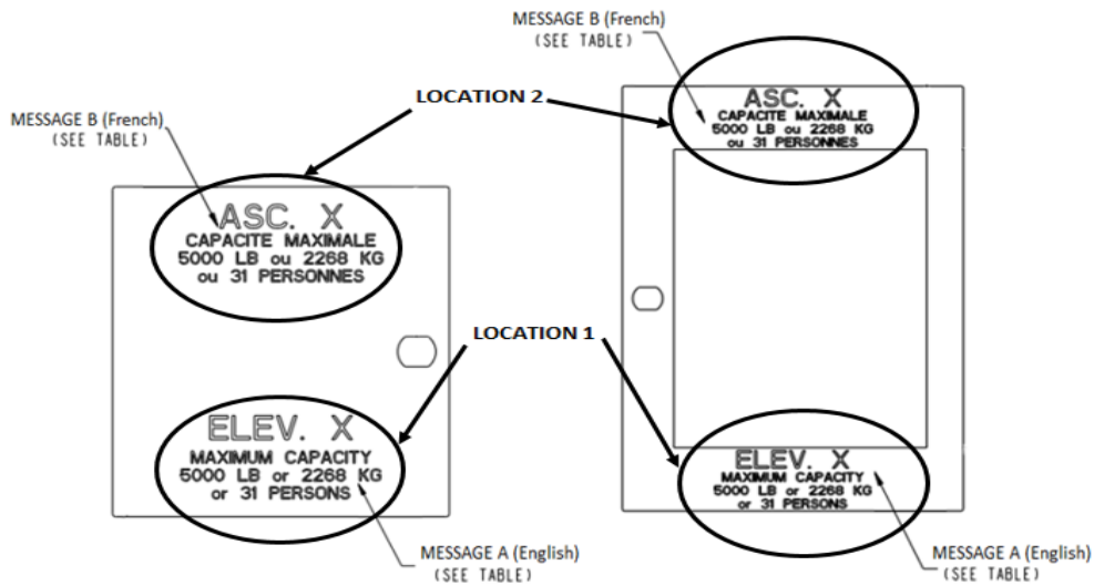
Door w/o Certificate window (LEFT HAND as shown)
