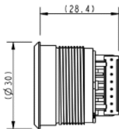
8 PIN AMP TERMINAL
