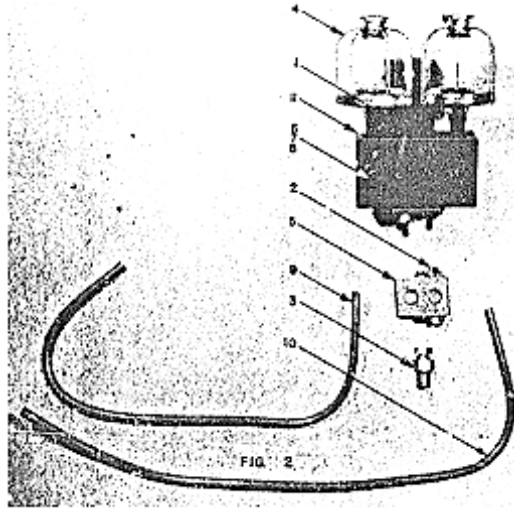
PARTS FOR STEP CHAIN LUBRICATOR - FIG. 2
