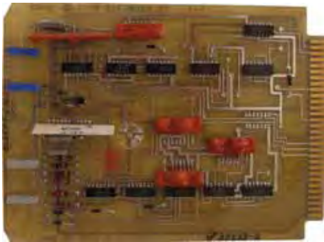
C8112B1 Car Variable 3 (CV3) Board
