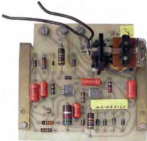
WEST195C252G01 PRD
