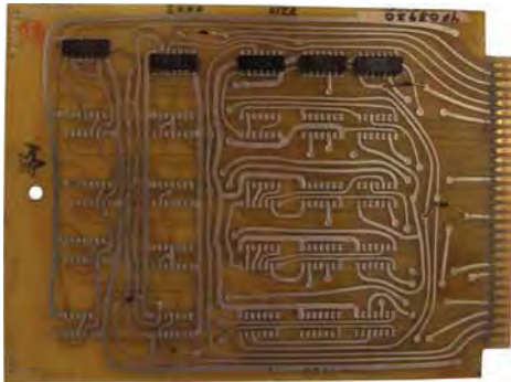
A8110A1 Board
